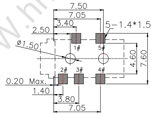
RECOMMENDED P.C.B LAYOUT TOP VIEW (TOLRANCE:±0.05)
